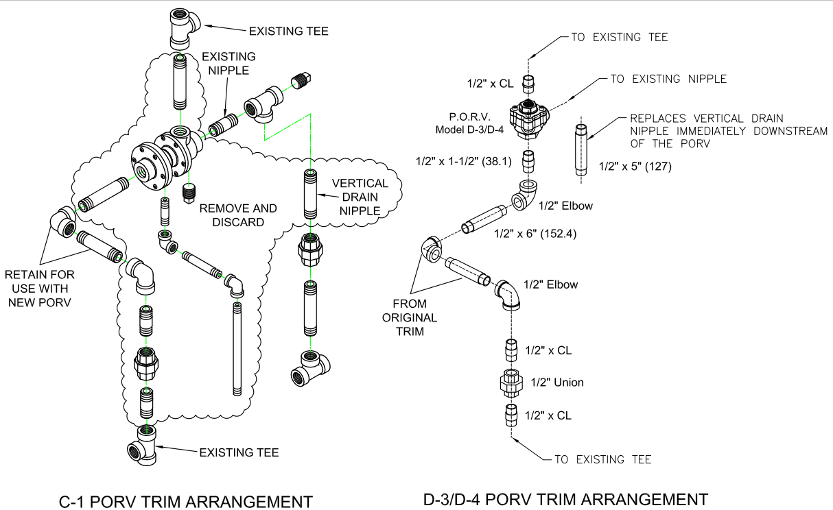
Figure 4 - Replacement PORV for Straight Through Horizontal Valves, 8"
