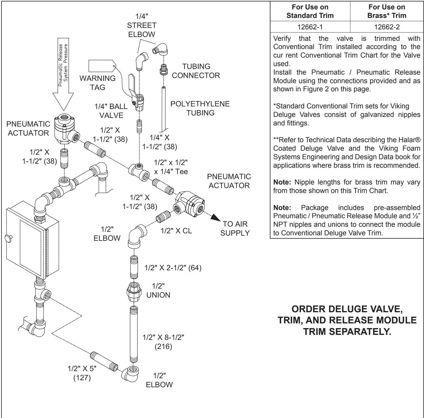
FIGURE 1: PNEUMATIC / PNEUMATIC RELEASE MODULE
