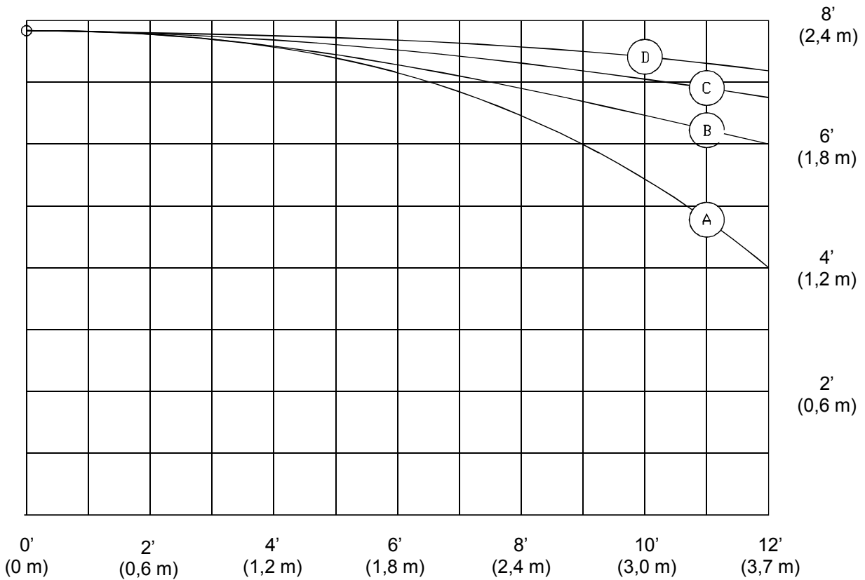
Typical front view of one half of the spray pattern produced by a 7/16" orifice Viking Model C-1 Window Sprinkler (4.3K) at a distance of 15" (381 mm) away from the window's surface.
