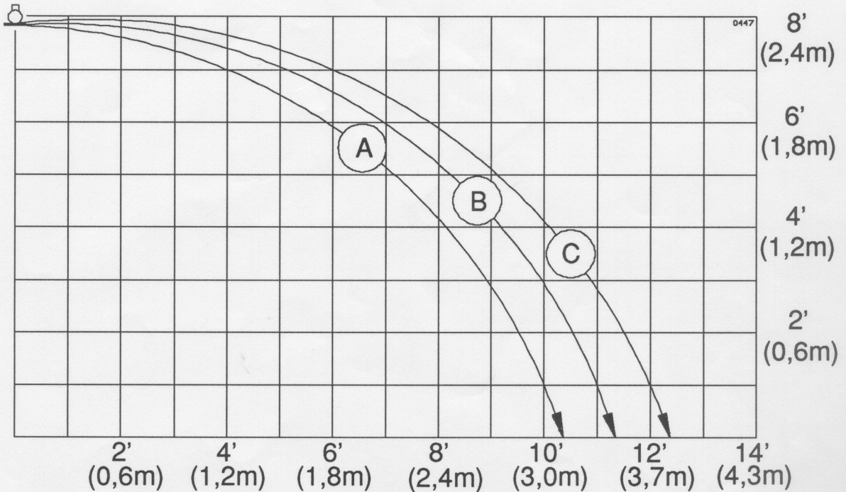
Typical profile of one half of the spray pattern produced by a Viking Micromatic Model M Dry Pendent Sprinkler (Plain Barrel).
