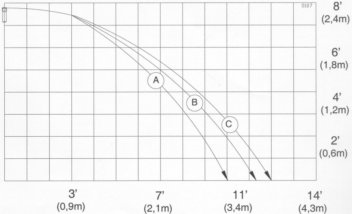
Typical profile of one half of the spray pattern produced by a Viking Model M Dry Upright Sprinkler.
