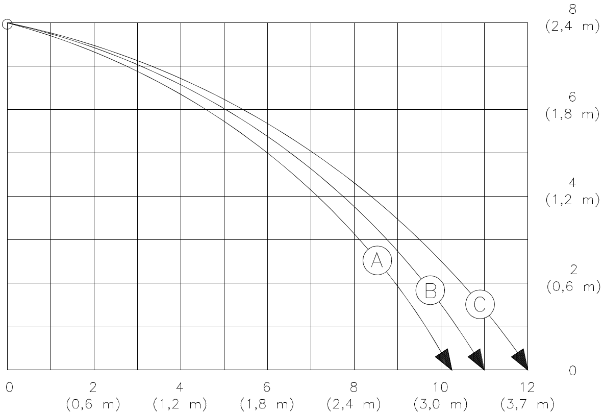
Typical profile of one half of the spray pattern produced by a Viking ELO Sprinkler SIN VK530 Sprinkler (K=11.2)
