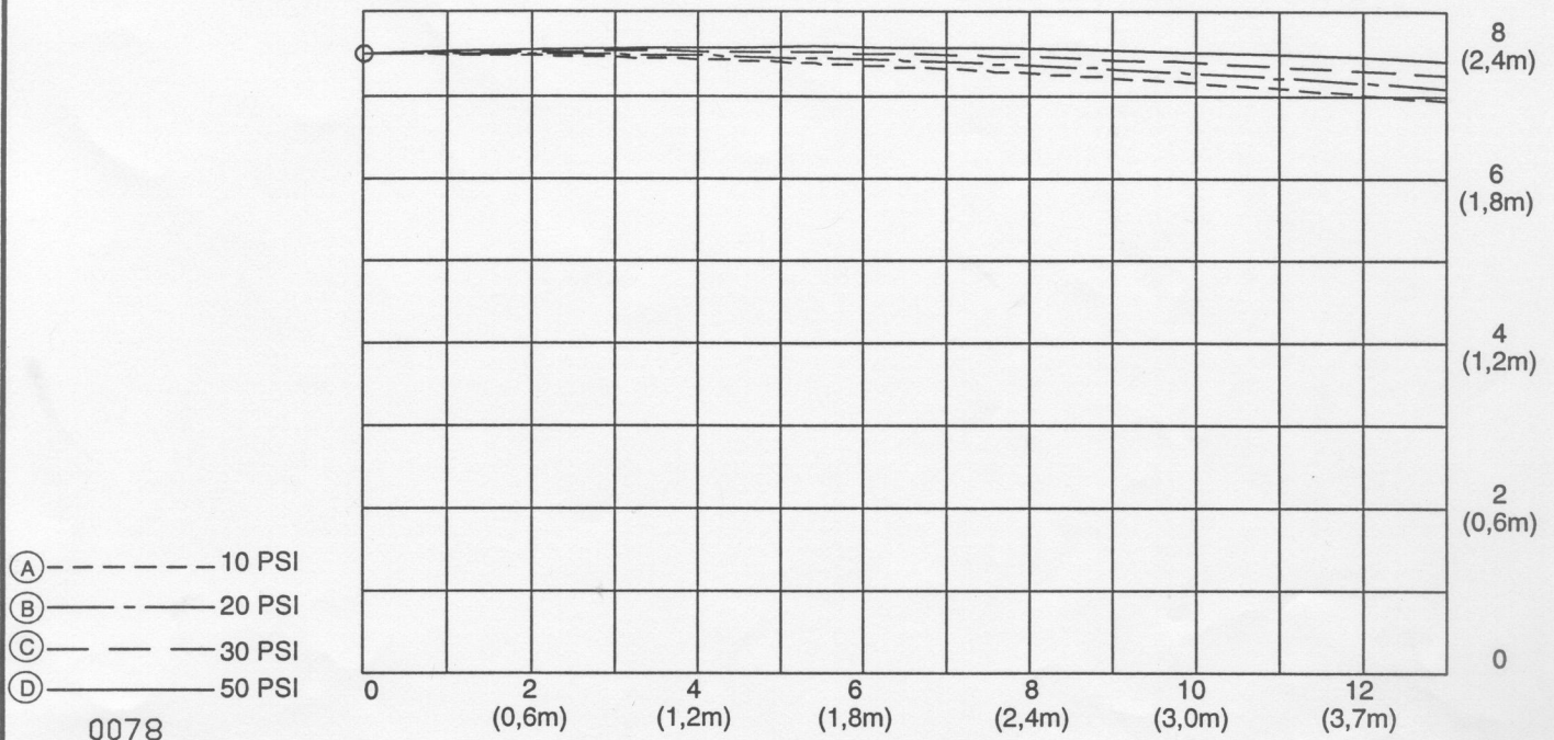
Typical front view of one half of the spray pattern produced by a 1/4" Viking Model C-1 Window Sprinkler at a distance of 15" (mm) away from the window's surface
