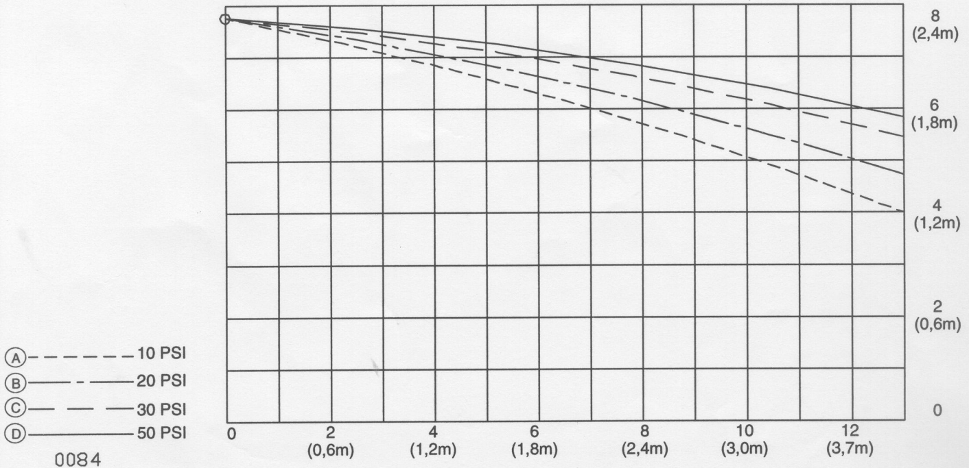
Typical front view of one half of the spray pattern produced by a 3/4" Viking Model C-1 Window Sprinkler at a distance of 15" (mm) away from the window's surface
