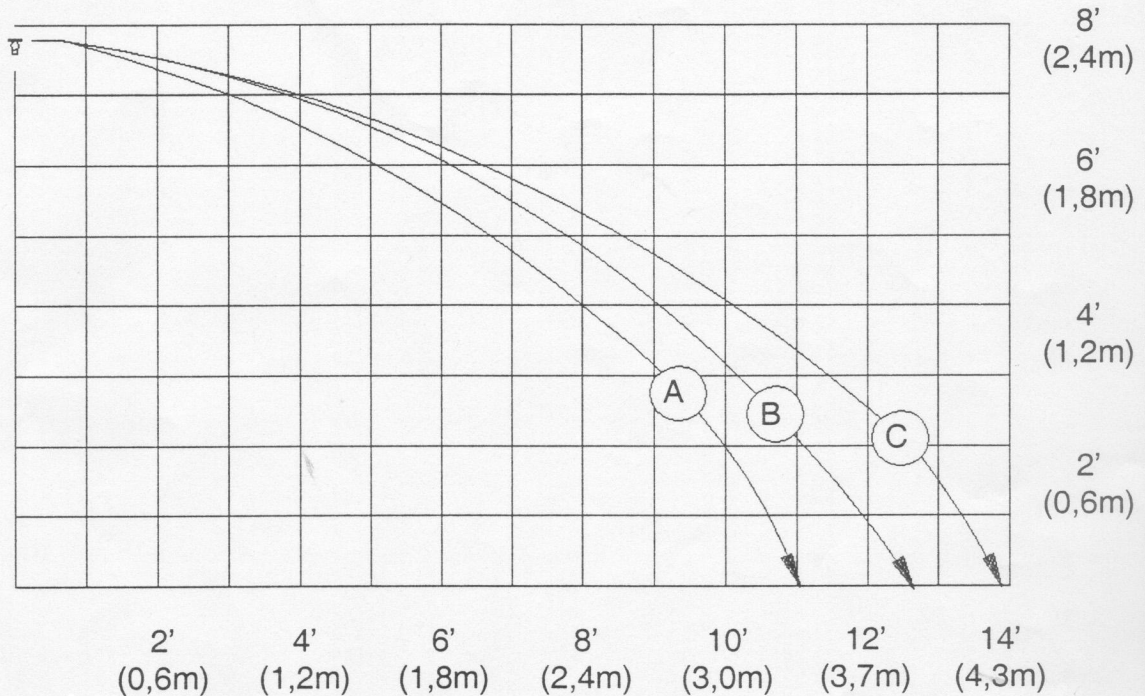
Typical profile of one half of the spray pattern produced by a Viking Model M 10mm (3/8") Orifice Upright Sprinkler
