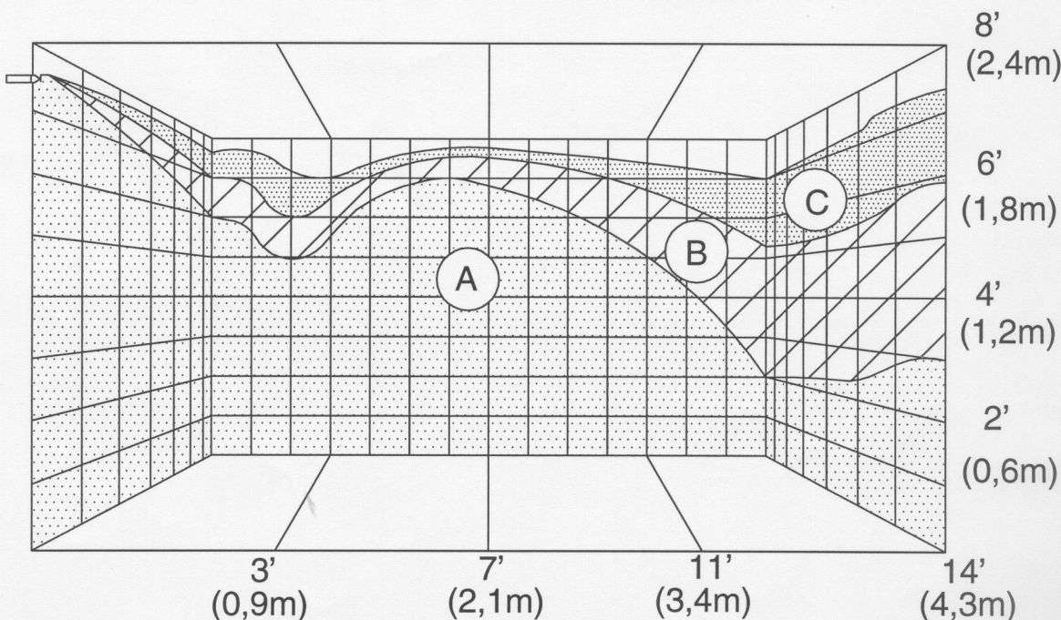
Typical profile of one half of the spray pattern produced by a Viking Model M Dry Horizontal Sidewall Sprinkler.
