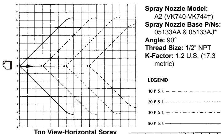
Top View-Horizontal Spray
