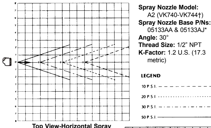
Top View-Horizontal Spray
