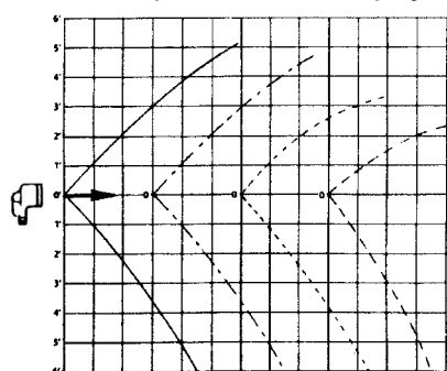
Top View-Horizontal Spray
