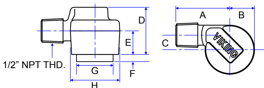
Figure 1: Spray Nozzle Dimensions
