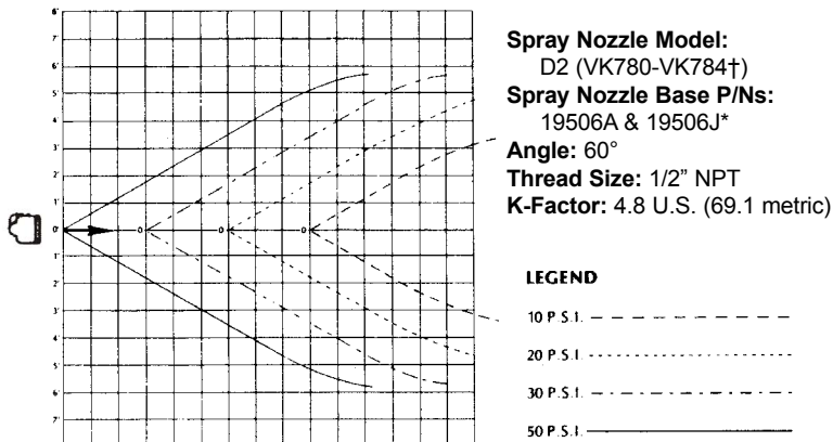
Top View-Horizontal Spray
