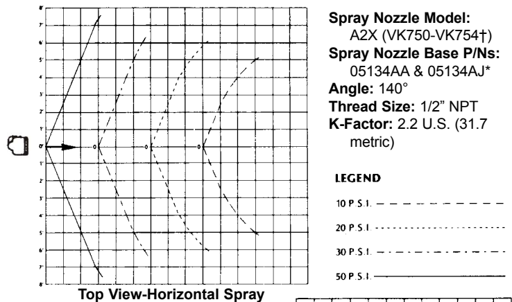
Top View-Horizontal Spray
