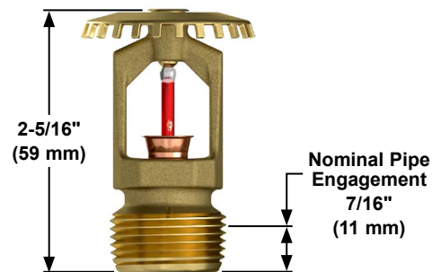
Figure 2: Sprinkler Dimensions
