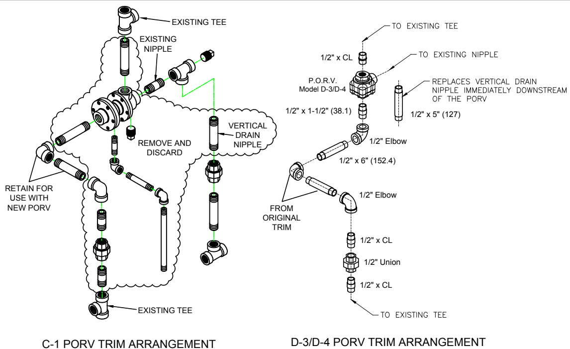
Figure 4 - Replacement PORV for Straight Through Horizontal Valves, 8"
