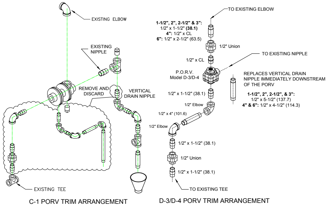
Figure 3 - Replacement PORV for Straight Through Horizontal Valves, Excluding 8"
