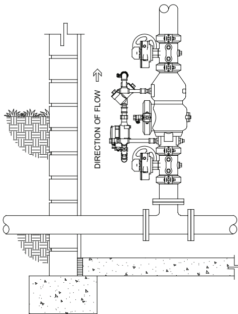
MODEL 350ADABG (Vertical Installation)
