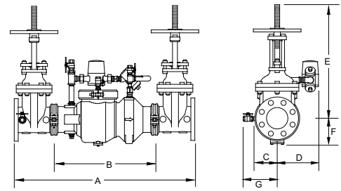
MODEL 350ADA with OS&Y option
