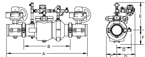
MODEL 350ADA with BG option
