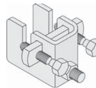
Fig. 825A Bar Joist Sway Brace Attachment Page 46
