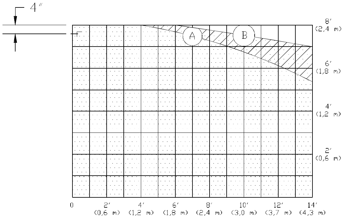
Typical side view of one half of the spray pattern produced by a Model H-4 Sidewall Sprinkler
