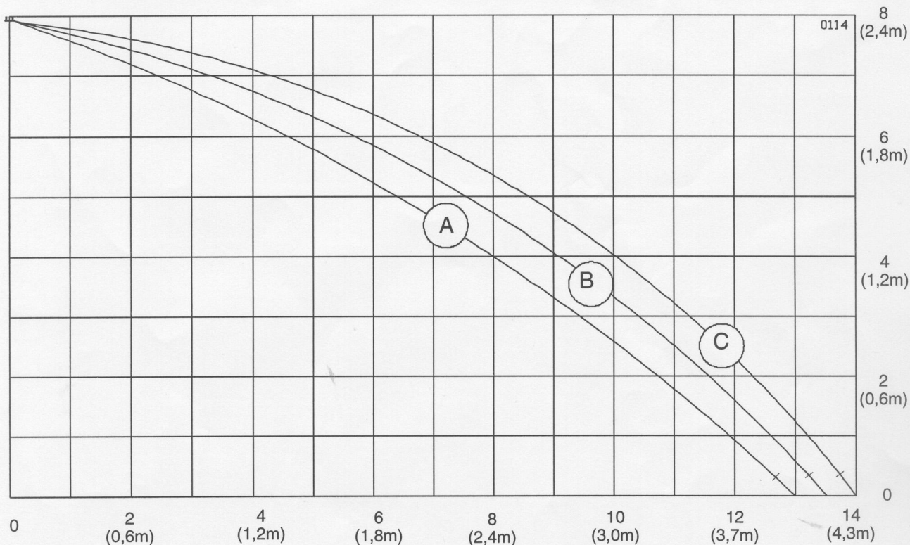
Typical front view of one half of the spray pattern produced by a Model B-1 Horizon Mirage Sprinkler
