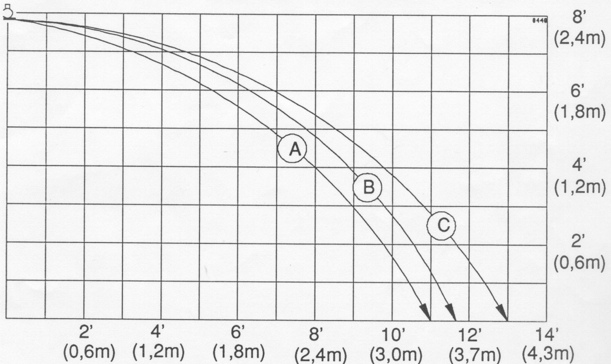
Typical profile of one half of the spray pattern produced by a Viking Micromatic Model M 3/8" Pendent Sprinkler.
