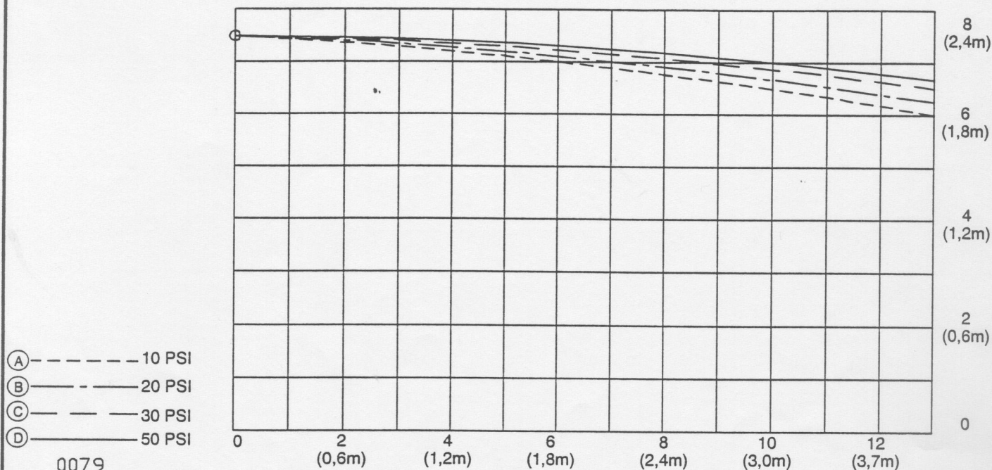
Typical front view of one half of the spray pattern produced by a 5/16" Viking Model C-1 Window Sprinkler at a distance of 15" (mm) away from the window's surface
