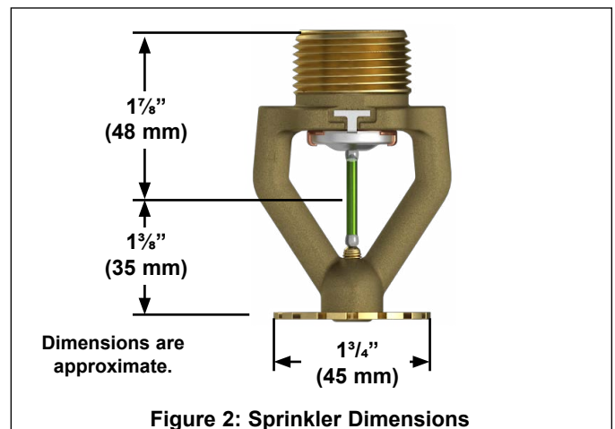
Figure 2: Sprinkler Dimensions
