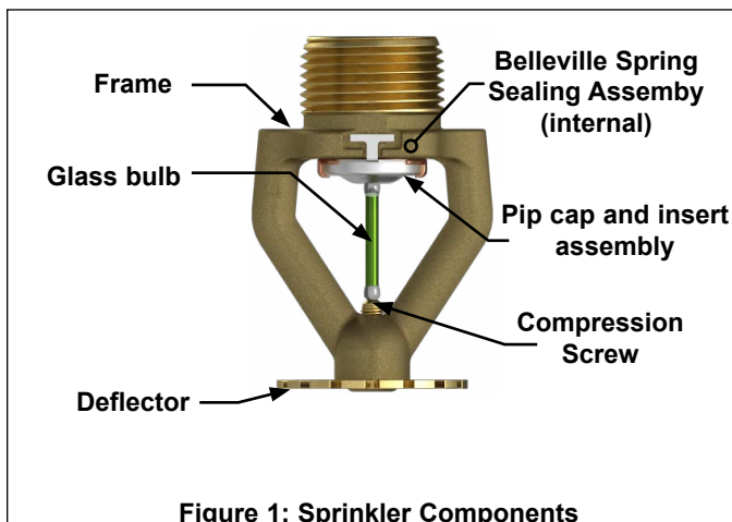
Figure 1: Sprinkler Components
