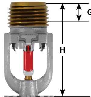
Figure – 2: Dimensions
