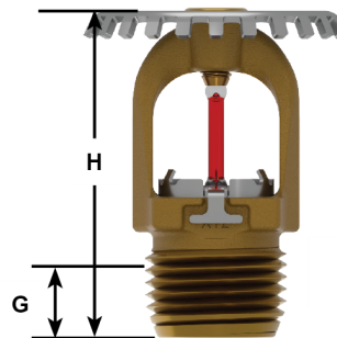
Figure – 2: Dimensions
