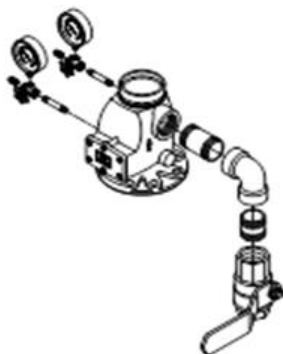
*2-1/2 - 6 inch trim shown
