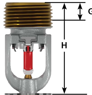
Figure - 2: Dimensions
