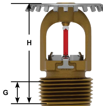
Figure – 2: Dimensions
