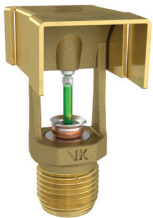
V-BB Back-to-Back 5.6 K-factor VK684, VK685, VK686
