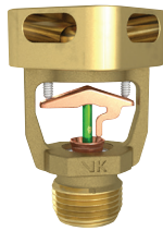
V-HIP Attic Hip 5.6 K-factor VK660
