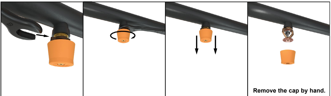
Figure 4: Sprinkler Installation
