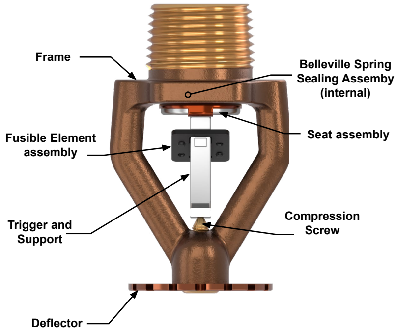
Figure 1: Sprinkler Components
