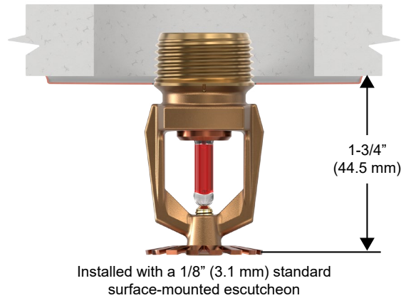
Figure 4: Sprinkler Dimensions
