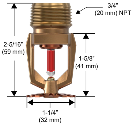
Figure 4: Sprinkler Dimensions
