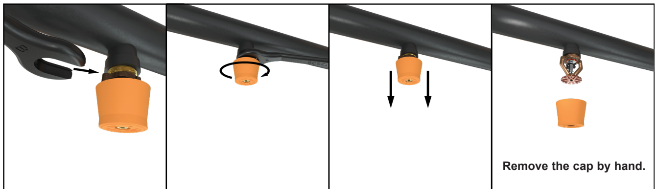
Figure 4: Sprinkler Installation
