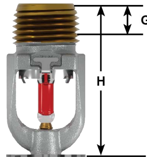
Figure – 2: Dimensions
