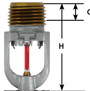
Figure – 2: Dimensions
