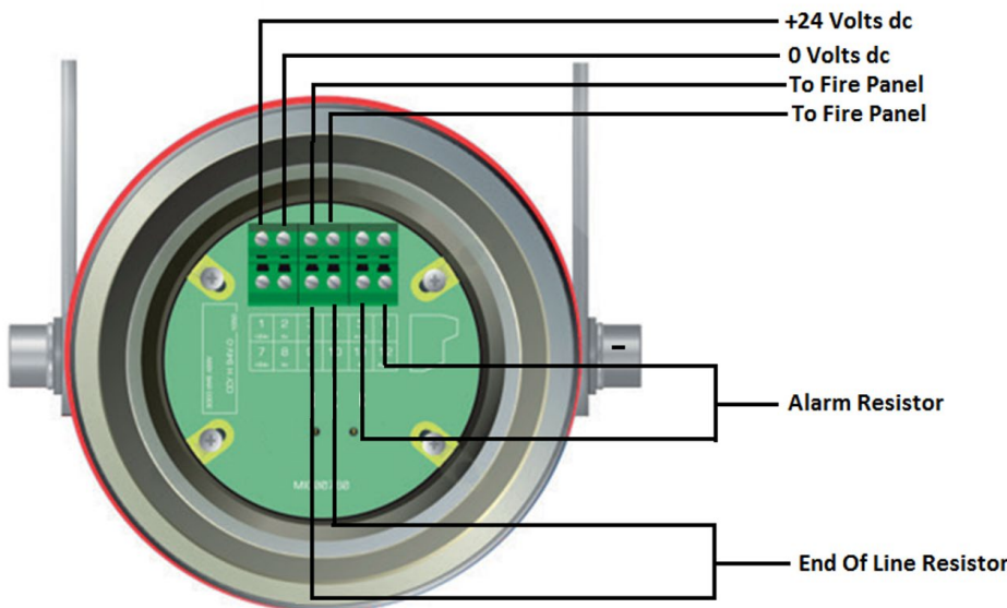
Figure 6: Relay Configuration Termination
