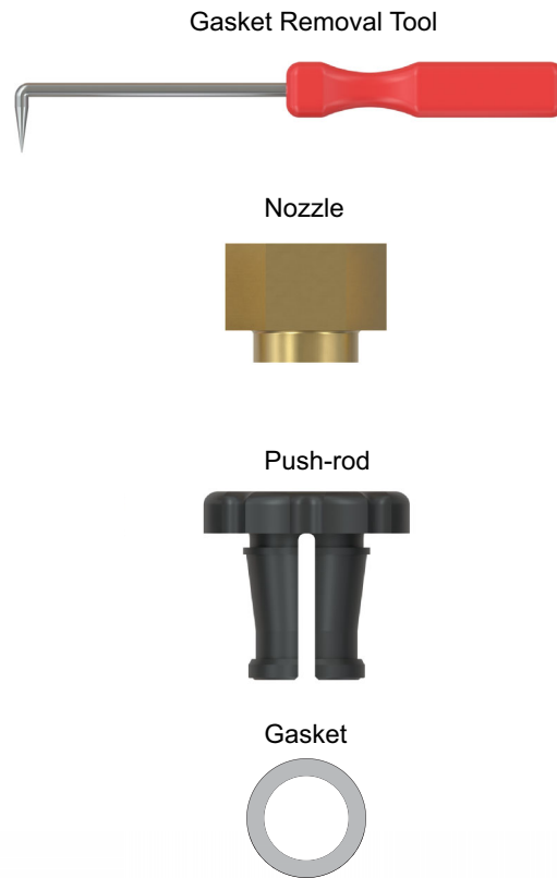
Figure – 1 Repair Kit Components
