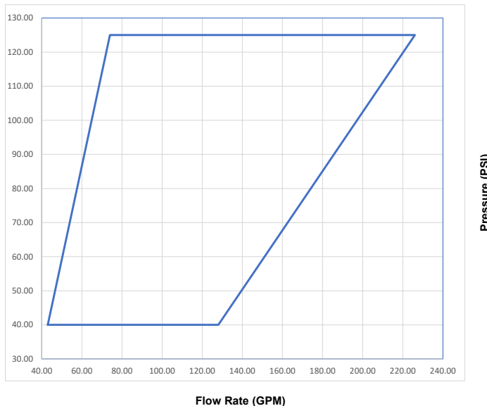
Graph 7.3.2 2.5" Model VFM With Viking ARK 3% | FM | Acetone
