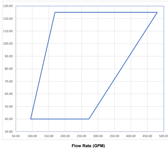
Graph 7.2.3 3" Model VFM With Viking ARK 3% | FM | IPA
