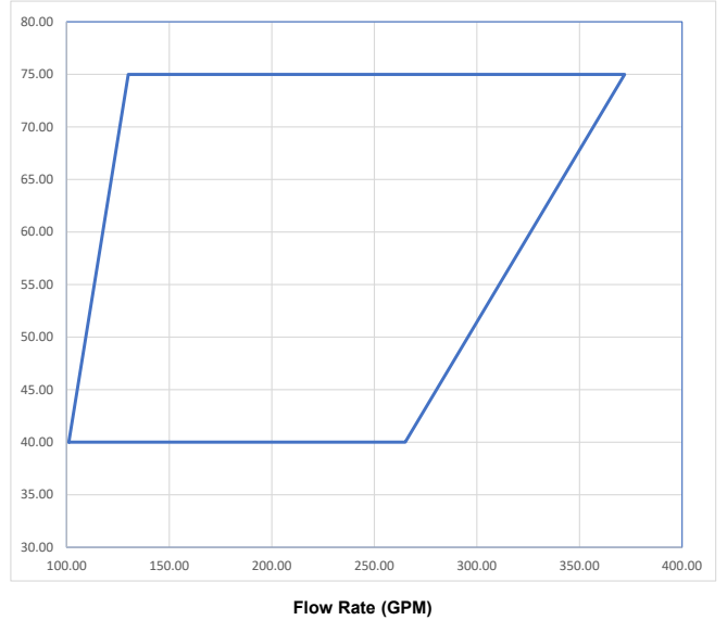
Graph 7.1.6 3" Model VFM With Viking USP 3% | FM | Heptane
