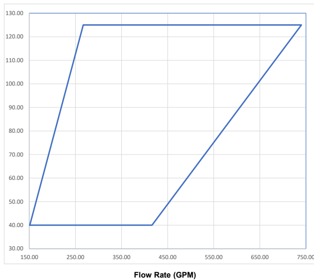
Graph 7.2.4 4" Model VFM With Viking ARK 3% | FM | IPA
