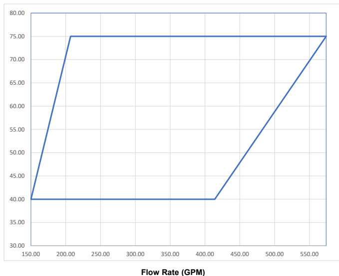
Graph 7.5.1 4" Model VFM With Viking USP 3% | FM | Jet A1
