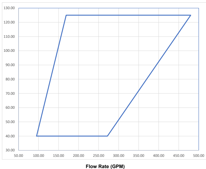
Graph 7.4.3 3" Model VFM With Viking ARK 3% | FM | Ethanol
