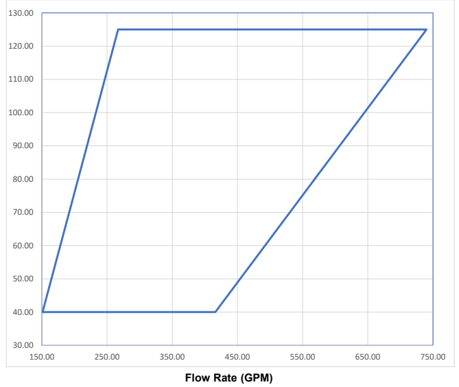
Graph 7.1.4 4" Model VFM With Viking ARK 3% | FM | Heptane
