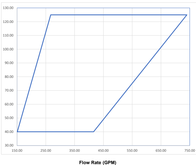
Graph 7.4.4 4" Model VFM With Viking ARK 3% | FM | Ethanol
