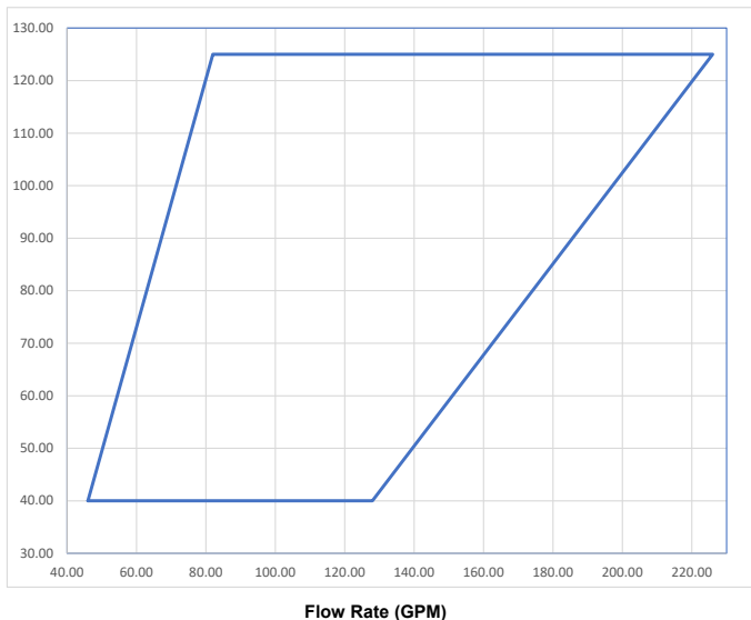
Graph 7.6.1 2.5" Model VFM With Viking USP 3% | UL | Hydrocarbons
