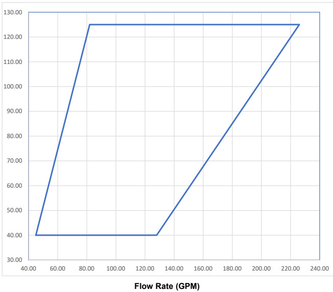
Graph 7.1.5 2.5" Model VFM With Viking USP 3% | FM | Heptane
