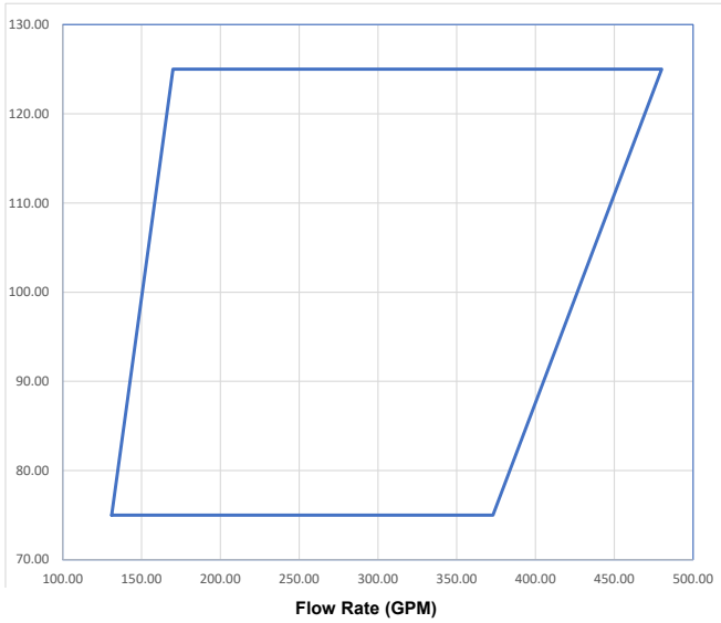
Graph 7.1.3 3" Model VFM With Viking ARK 3% | FM | Heptane
