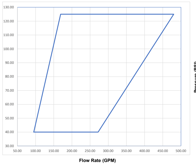
Graph 7.3.3 3" Model VFM With Viking ARK 3% | FM | Acetone
