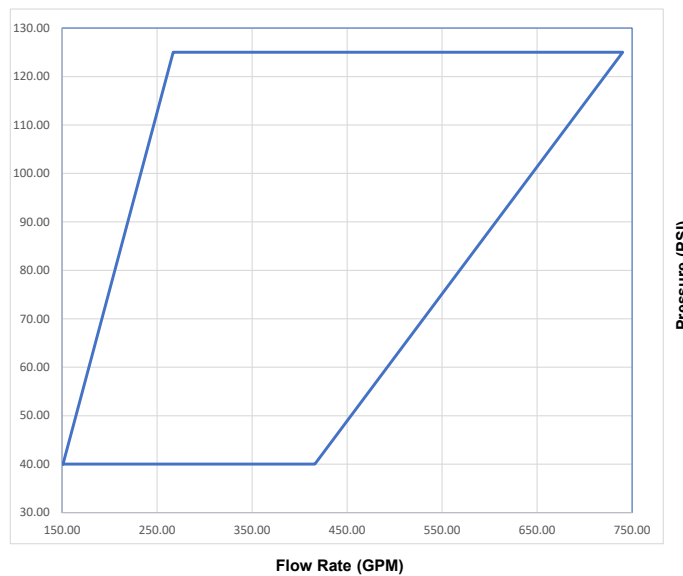
Graph 7.3.4 4" Model VFM With Viking ARK 3% | FM | Acetone
