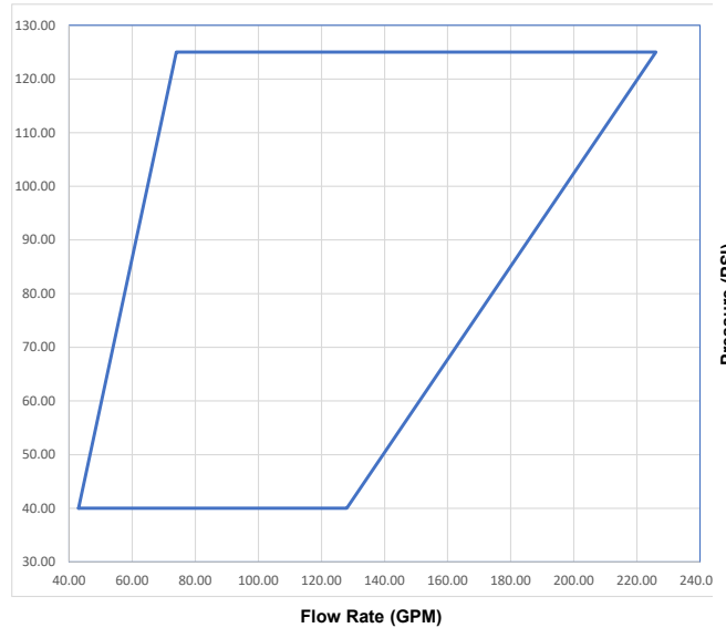
2.5" Model VFM With Viking ARK 3% | FM | Heptane
