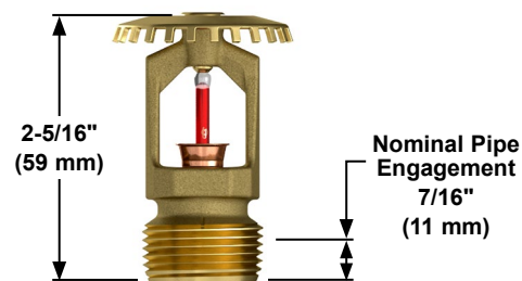
Figure 2: Sprinkler Dimensions
