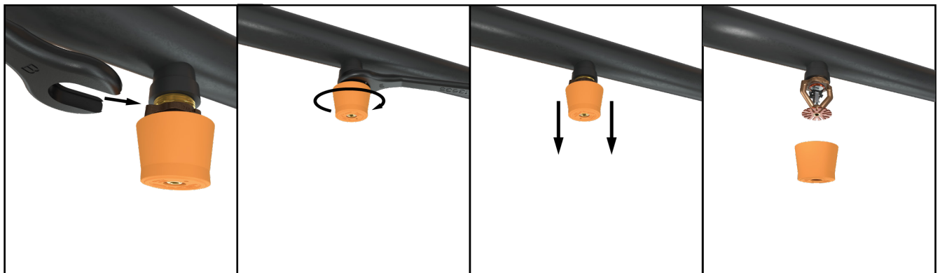
Figure 4: Sprinkler Installation
