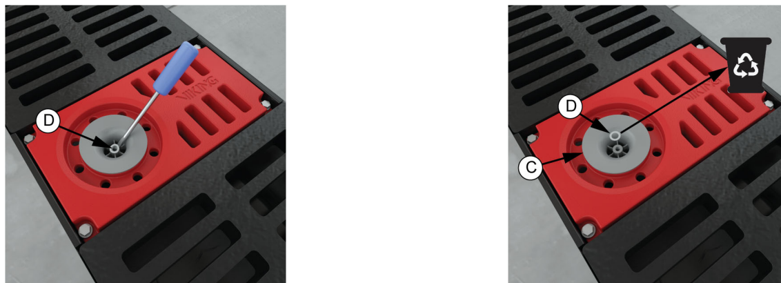
Figure – 5 Removing the Existing PTFE Washer
