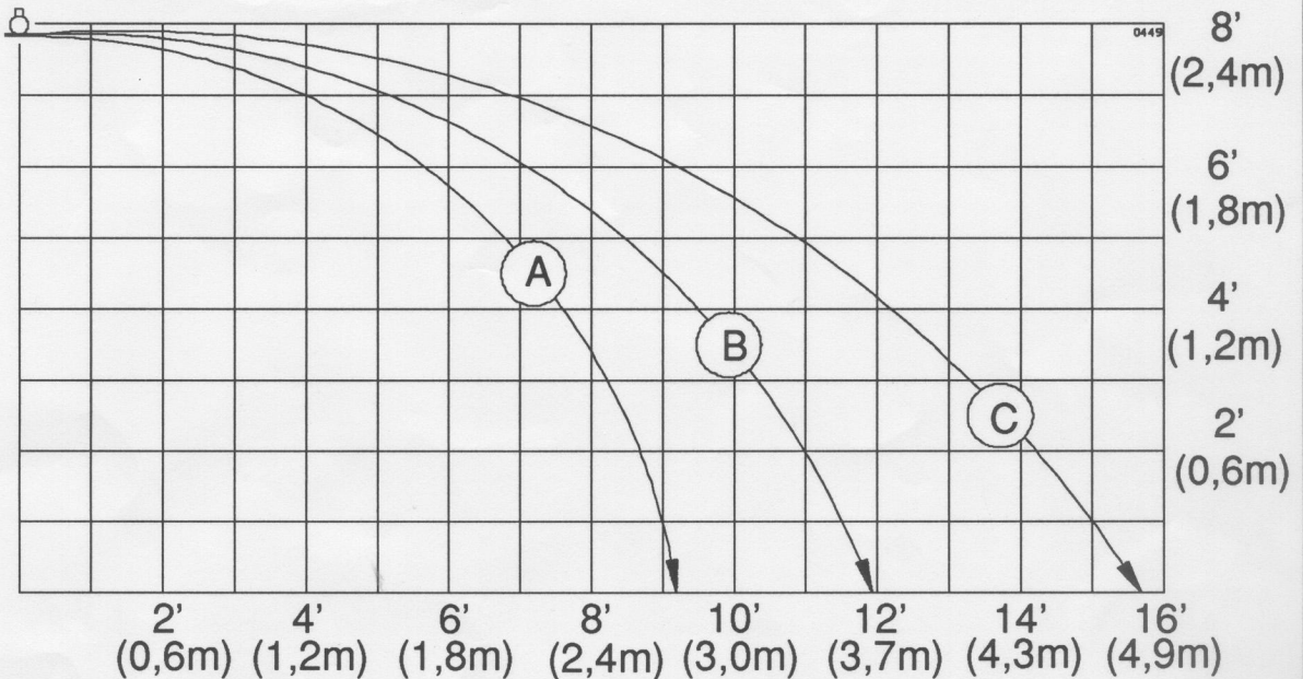
Typical profile of one half of the spray pattern produced by a Viking Microfast Model M 1/2" (15mm) Orifice Extended Coverage Pendent Sprinkler.
