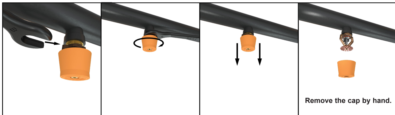
Figure 4: Sprinkler Installation
