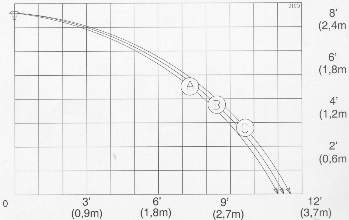
Typical profile of one half of the spray pattern produced by a Viking Model A-2 Hi-Challenge Large Drop Sprinkler
