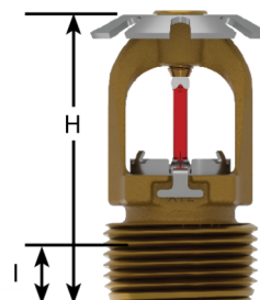
Figure – 2: Dimensions
