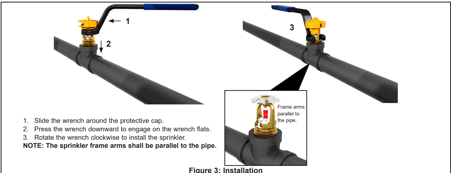
Figure 3: Installation
