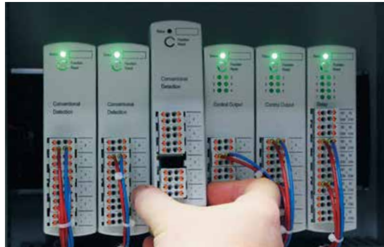
HOT SWAP module exchange
