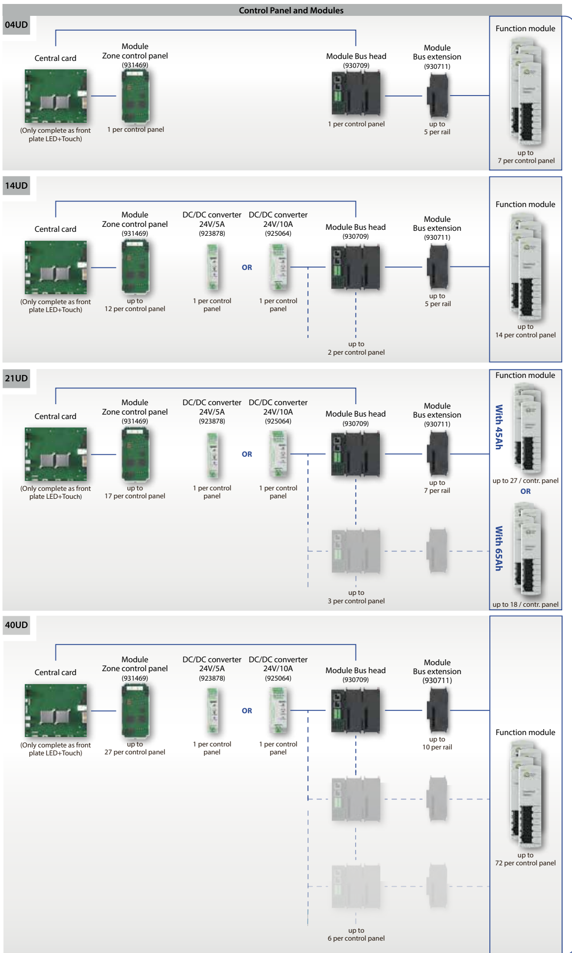
Clunid DCP-1 - Panel functions & Module extension
